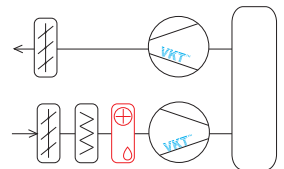
Схема 1.2 VAC-W-ShD1D3D3D35D125D14T123
