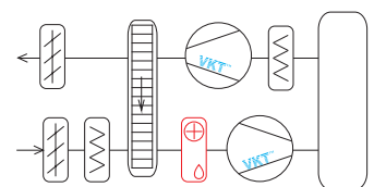
Схема 1.2 VAC-W-ShD1D3D3D35D125D14T123
