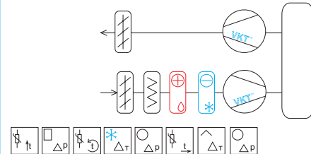
Схема 5.2 VAC-WF-ShD1D3D3D35D125D14T123Kt
