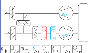
Схема 5.3 VAC-WF-ShD1D3D3D35D125D14T123Kt
