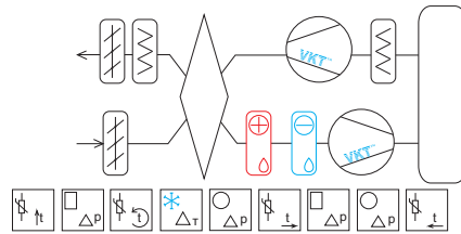
Схема 4.4 VAC-WO-ShD1D1D3D3D35D35D125D14T123
