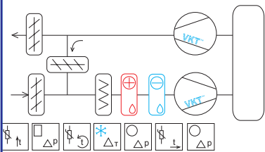
Схема 4.3 VAC-WO-ShD1D3D3D35D125D14T123
