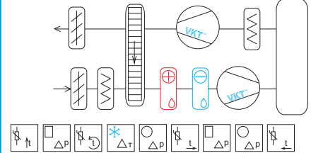
Схема 4.5 VAC-WO-ShD1D1D3D3D35D35D125D14T123
