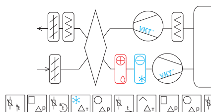
Схема 5.4 VAC-WF-ShD1D1D3D3D35D35D125D14T123Kt
