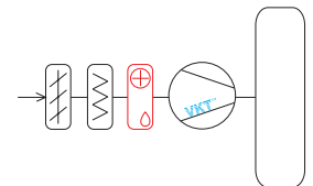
Схема 1.1 VAC-W-ShD1D3D3D35D125D14T123
