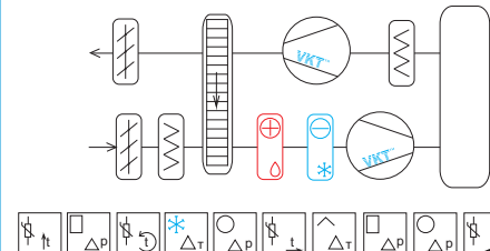
Схема 5.5 VAC-WF-ShD1D1D3D3D35D35D125D14T123Kt
